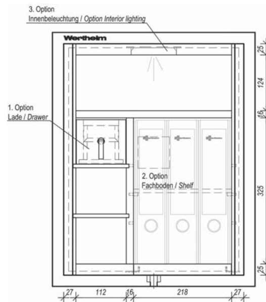
View from drawing ALZ 007 200
